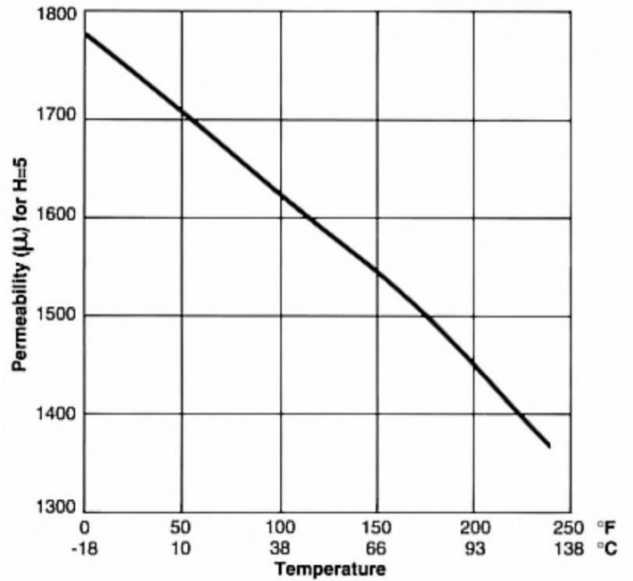
Permeability vs Temperature Characteristics – Invar 36
