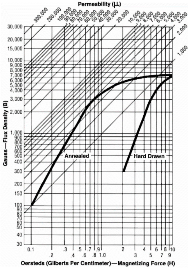
DC Magnetic Permeability Curves – Invar 36
